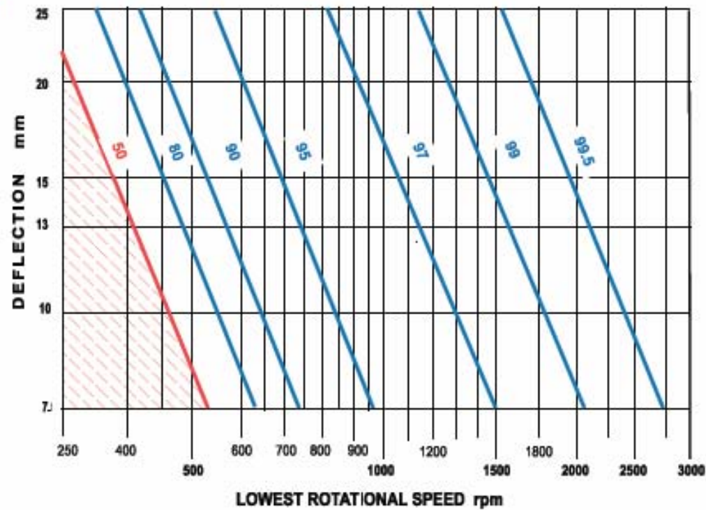
ISOLATION EFFICIENCY %
