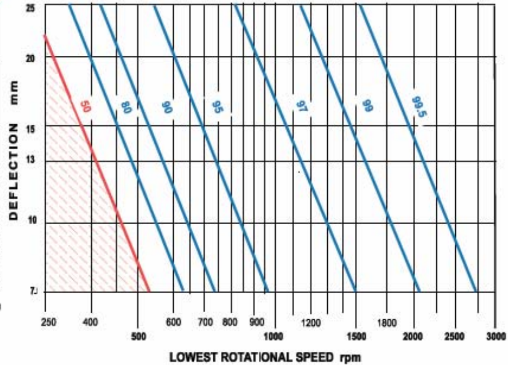
ISOLATION EFFICIENCY %
